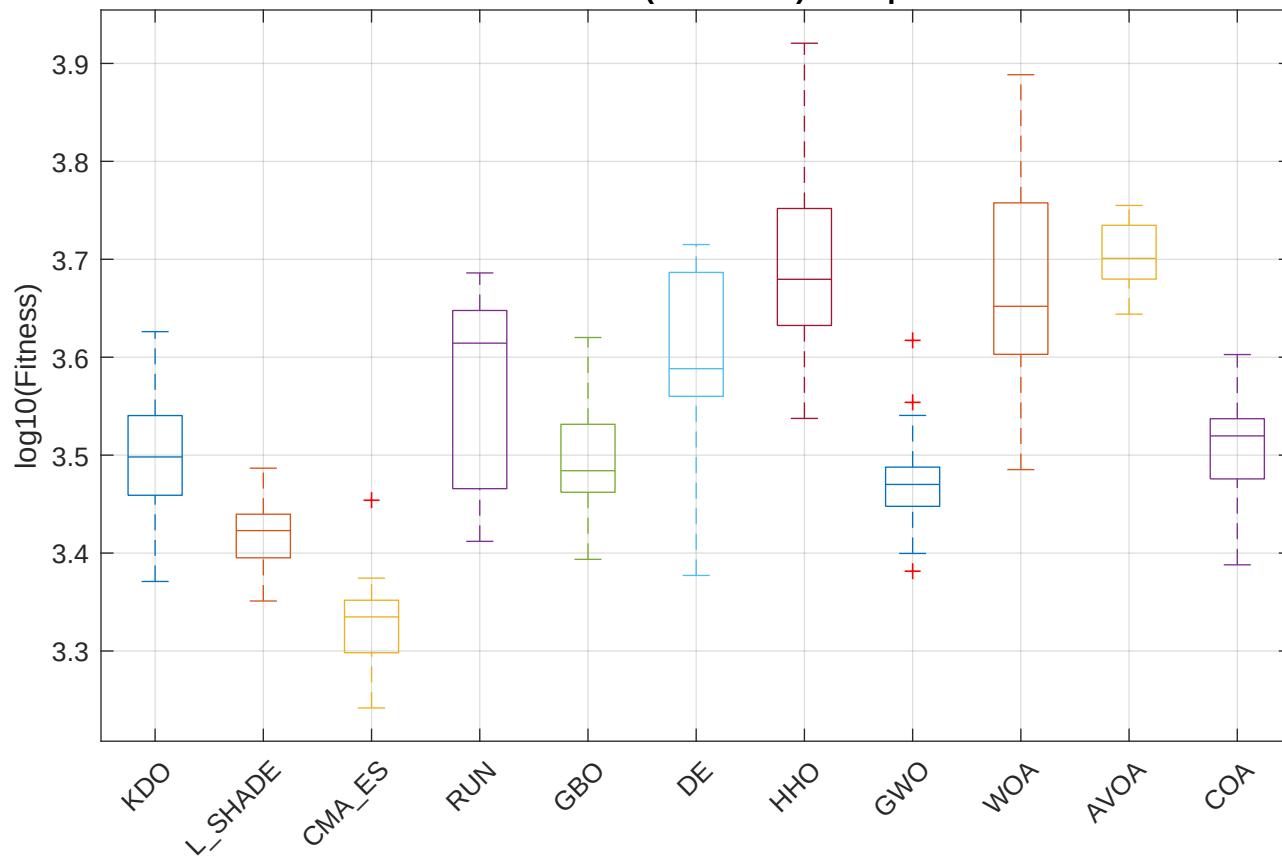
CEC2017 F16 (Numerical) - Boxplot
